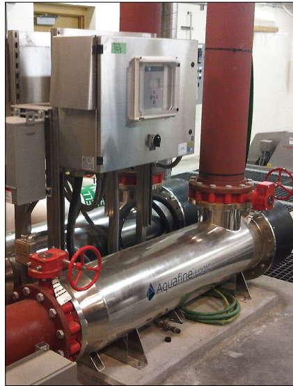
The highly efficient "L-shaped" design and low-pressure, high-output (LPHO) amalgam lamps result in an extremely compact footprint.
